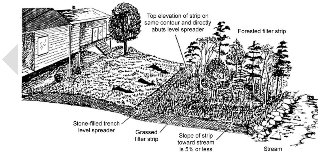
Figure 28: Filter Strip Incorporating Grassed and Wooded Areas (Cited by Barr Engineering, Co., 2001; Source: Claytor, 1996)
