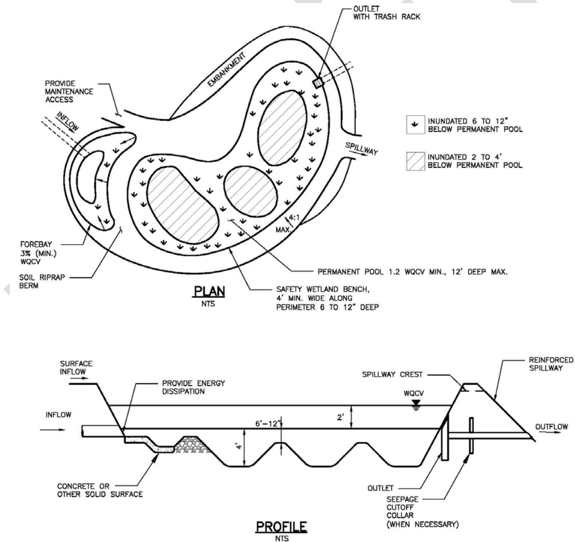
Figure 6: Plan and Profile View of a Constructed Wetland (Source: UDFCD, 2010)
